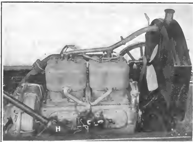
Fig. 2—Water and gas manifolds are cast integrally
